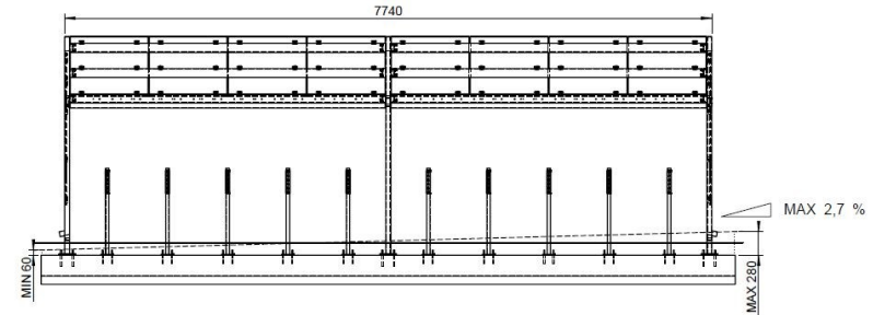
KUBATURA BETONU / CONCRETE CUBATURE / BETONRAUMINHALT 8.31m 3
