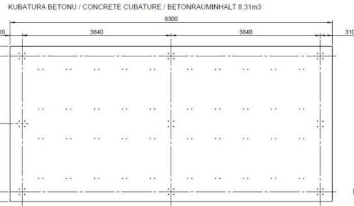
KUBATURA BETONU / CONCRETE CUBATURE / BETONRAUMINHALT 8.31m 3
